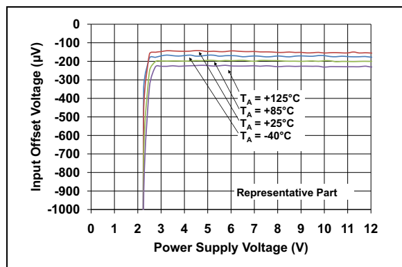
FIGURE 2-7: Input Offset Voltage vs. Power Supply Voltage.
