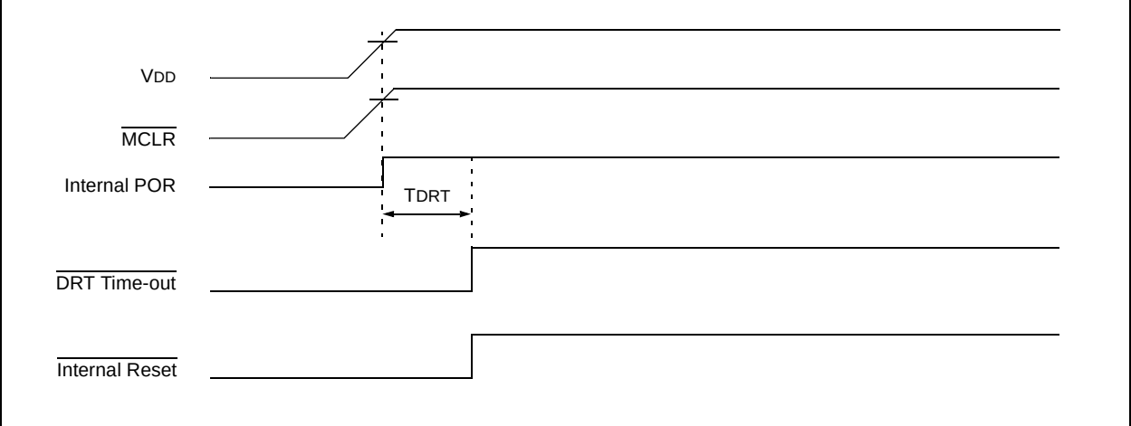
FIGURE 5-5: TIME-OUT SEQUENCE ON POWER-UP ( \overline{\text{MCLR}} TIED TO V_{DD} ): SLOW V_{DD} RISE TIME
