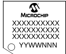
44-Lead TQFP
