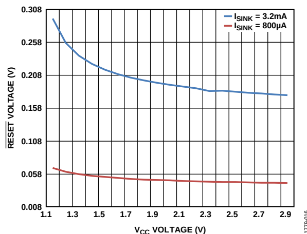
Figure 16. \overline{RESET} Open-Drain V_{OL} Voltage vs. V_{CC} Voltage ( V_{TH} = 3 V )
