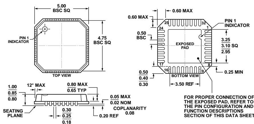
Figure 71. 32-Lead Lead Frame Chip Scale Package [LFCSP_VQ]
