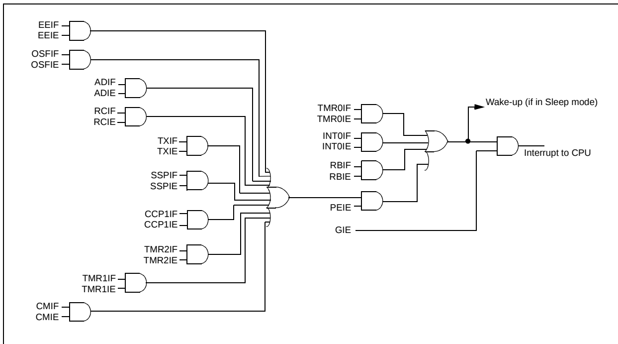
FIGURE 15-7: INTERRUPT LOGIC
