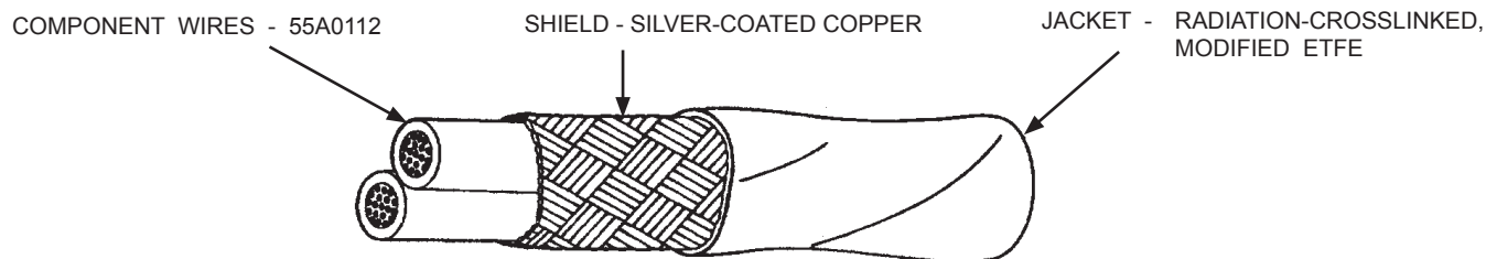
CABLE CONSTRUCTION DETAILS
