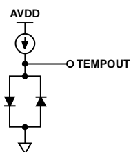
Figure 31. Equivalent TEMPOUT Output Circuit
