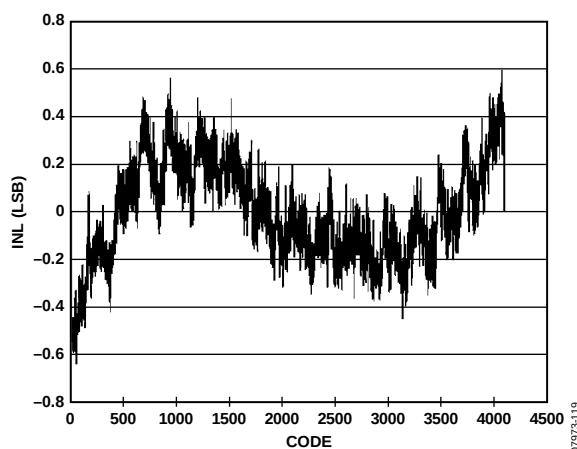
Figure 19. INL, f_{\text{IN}} = 9.7 \text{ MHz} , f_{\text{SAMPLE}} = 210 \text{ MSPS}
