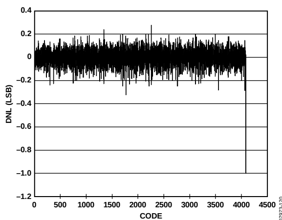
Figure 20. DNL, f_{\text{IN}} = 9.7 \text{ MHz} , f_{\text{SAMPLE}} = 210 \text{ MSPS}
