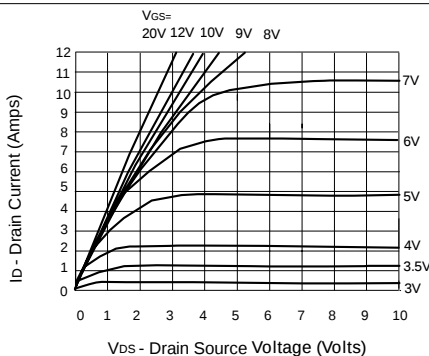
Saturation Characteristics
