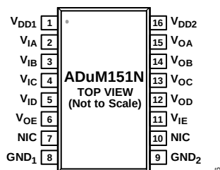
Figure 6. ADuM151N Pin Configuration
