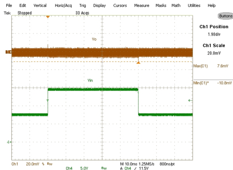
Fig (16) Feed Forward for V_{in} change from 6.8 to 16V and back to 6.8V Ch 1 - V_o Ch 4 - V_{in}
