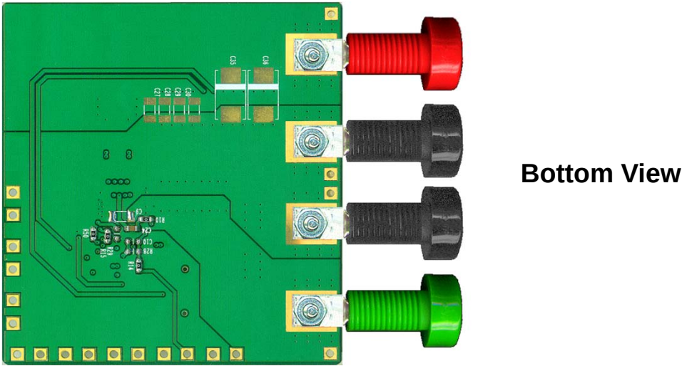
Fig. 1: Connection Diagram of IR3895/94 Evaluation Boards
