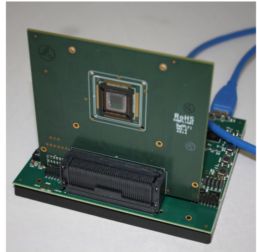
Figure 1. PYTHON Image Sensor Evaluation Board
