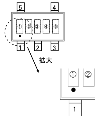
SOT-25(Under dot)
