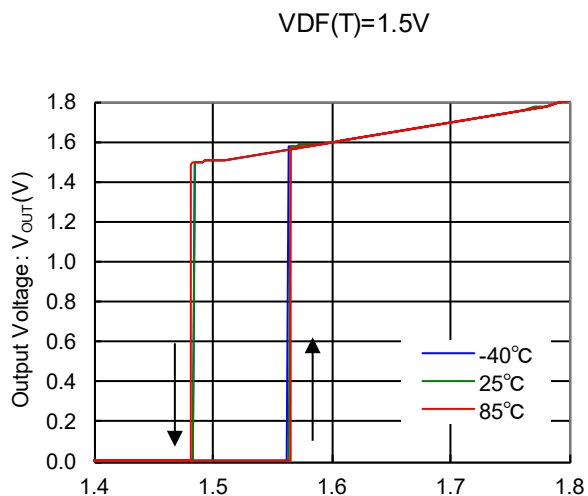
(3) Output Voltage vs. Input Voltage
