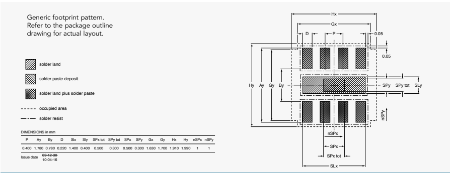
DFN1714U-8 (SOT983)
