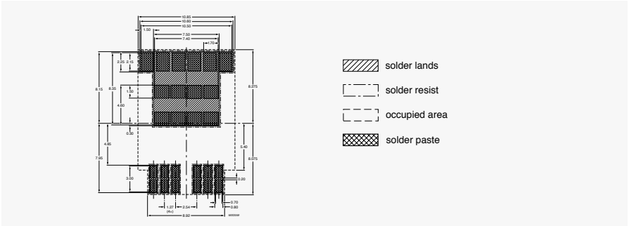
D2PAK-7 (SOT428)
