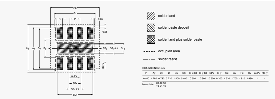
DFN1714-8 (SOT1166)
