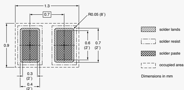
DFN1006-2 (SOD882)
