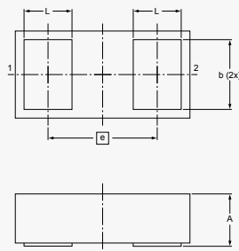
DSN0402-2 (SOD992)
