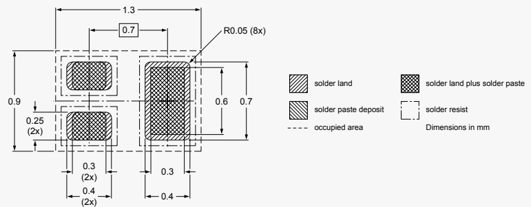
DFN1006B-3 (SOT883B)
