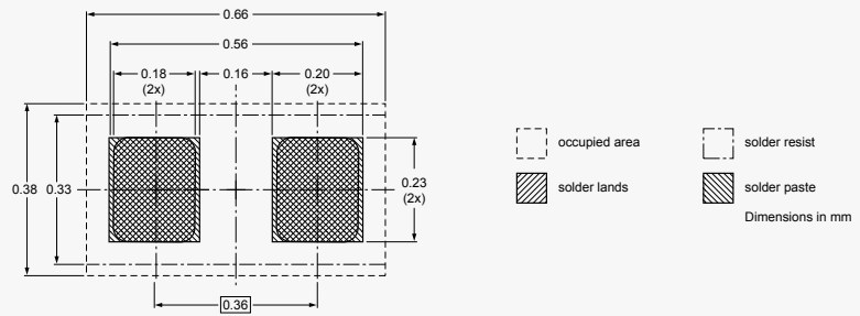
DSN0402-2 (SOD992)
