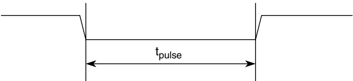
Figure 2-48. Pulse Illustration
