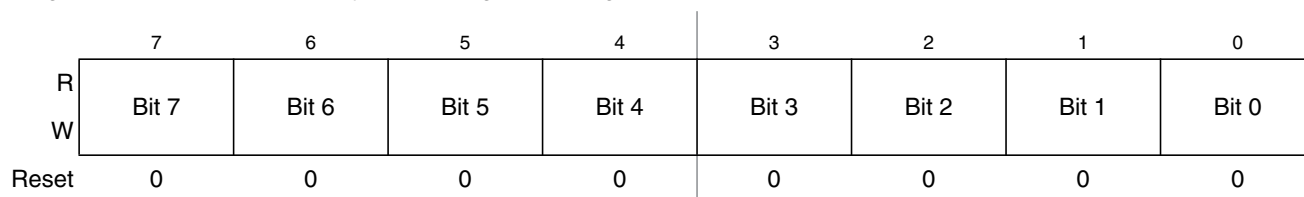
Figure 7-18. Debug Comparator A Register Low (DBGCAL)
