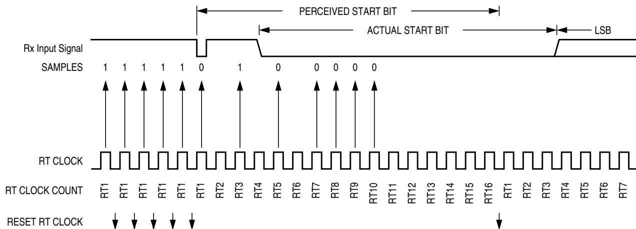
In Figure 13-15, verification sample at RT3 is high. The RT3 sample sets the noise flag. Although the perceived bit time is misaligned, the data samples RT8, RT9, and RT10 are within the bit time and data recovery is successful.
