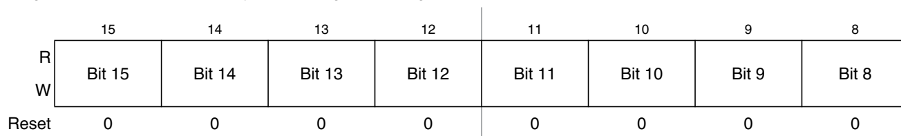
Figure 7-17. Debug Comparator A Register High (DBGCAH)
