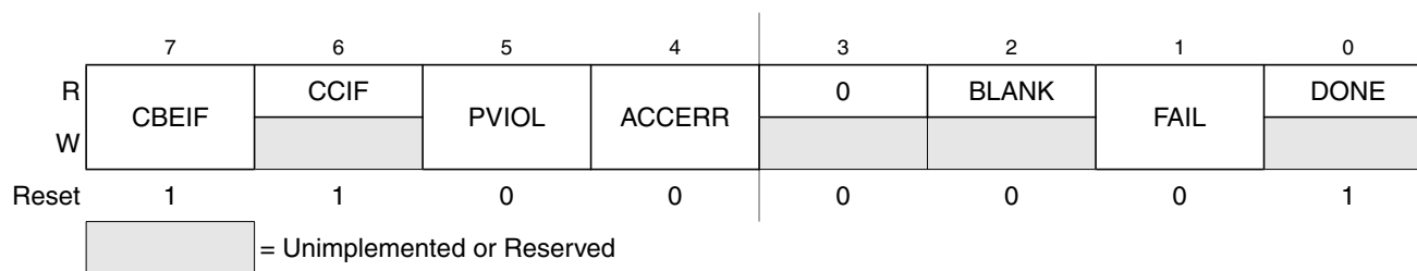
Figure 19-12. Flash Status Register (FSTAT)
