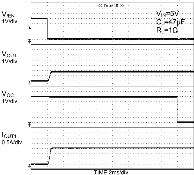
Figure 36. Over-Current Response Enable to 1Ω short (BD2062FJ)
