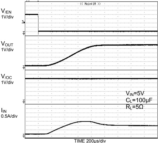
Figure 30. Output Rise Characteristics (BD2062FJ)
