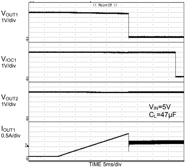
Figure 34. Over-Current Response Ramped Load (BD2062FJ)
