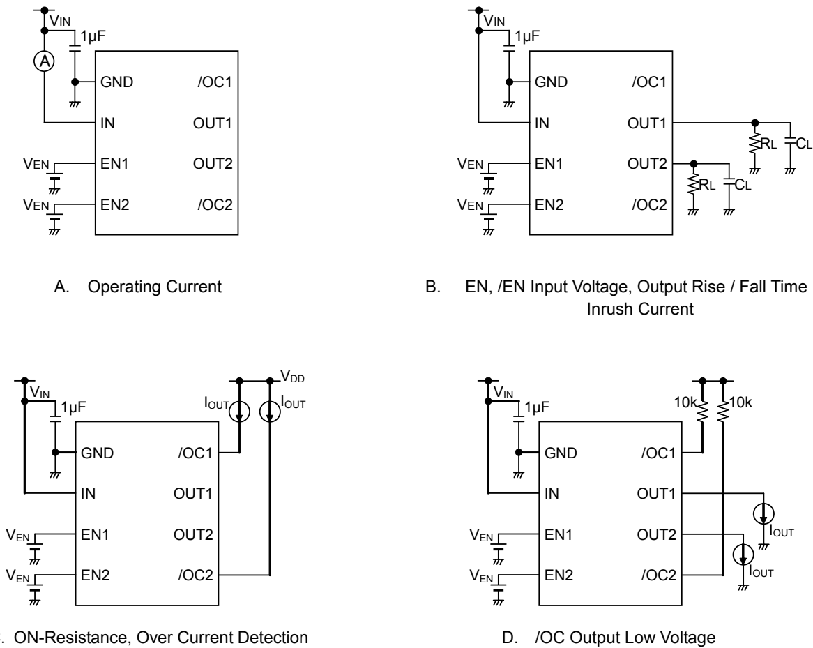
Figure 1. Measurement Circuit
