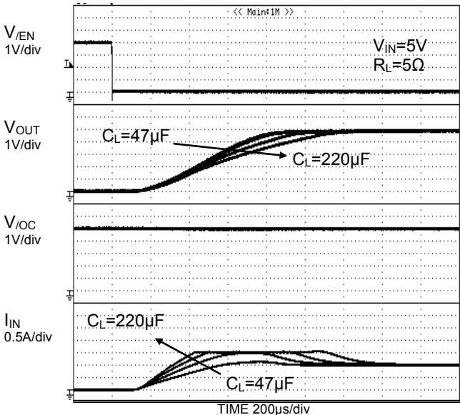
Figure 32. Inrush Current C_L=47\mu\text{F} , 100\mu\text{F} , 147\mu\text{F} , 220\mu\text{F} (BD2062FJ)
