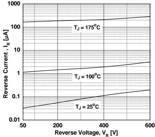
Figure 23. Reverse Current
