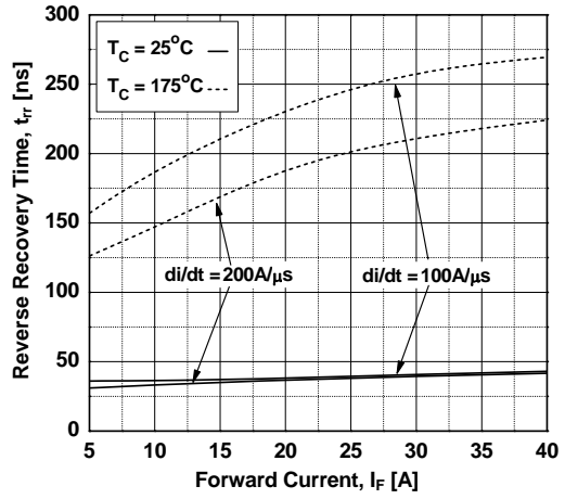
Figure 26. Reverse Recovery Time, t_{rr} [ns]
