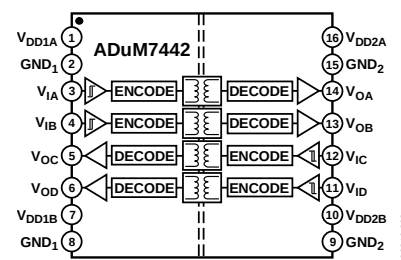
Figure 3. ADuM7442
