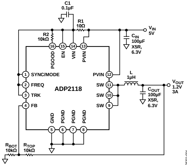
Figure 41. Application Circuit
