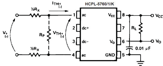
Figure 11. External threshold voltage level selection.
