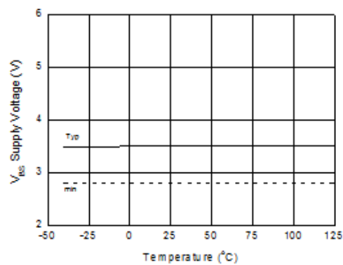
Figure 50. V_{BS} Under-Voltage Threshold (-) vs. Temperature
