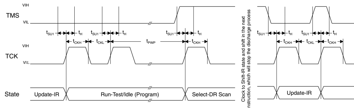
Figure 2-4. Programming Timing Diagram
