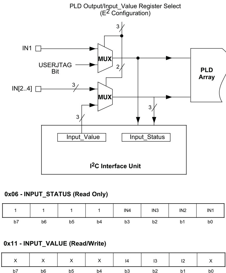
Figure 2-20. I 2 C Digital Input Interface
