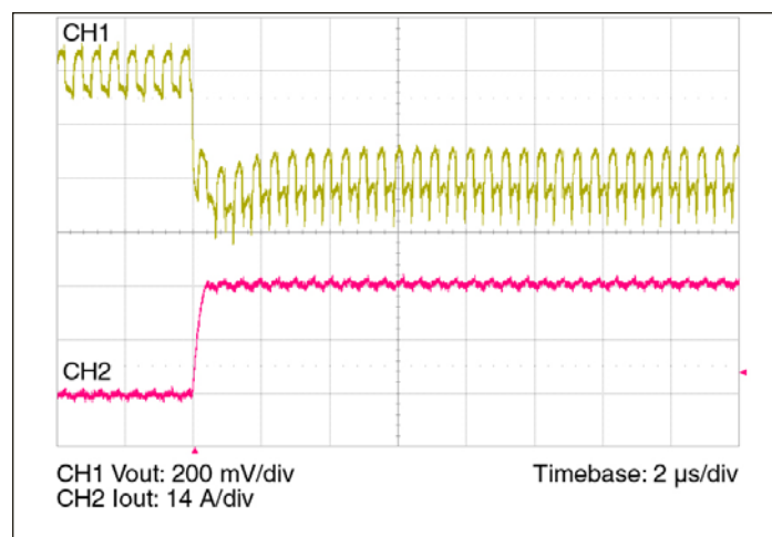
Figure 10 — 0-28.0 A load step with 2 \mu F input capacitor and no output capacitor.
