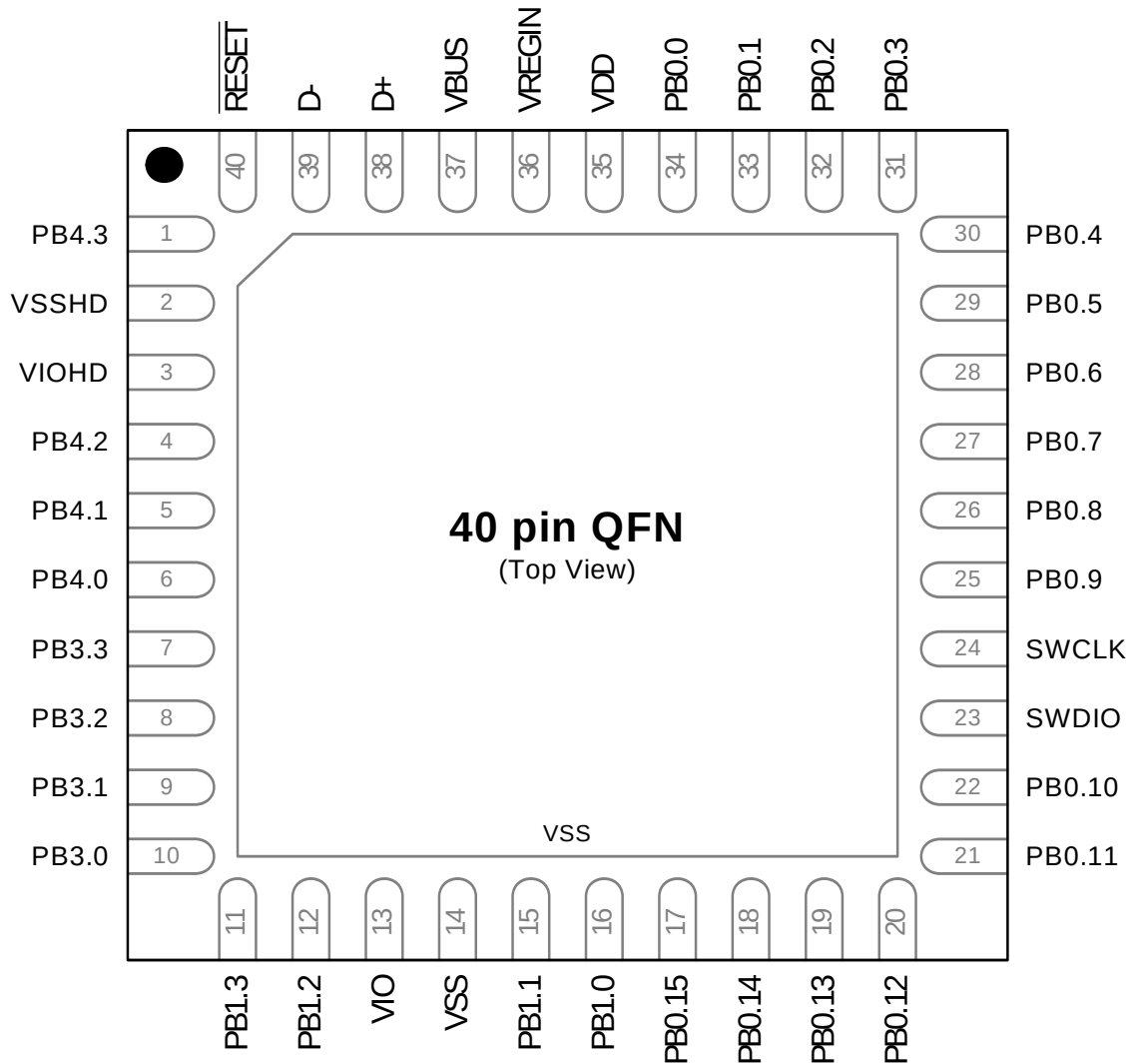
Figure 6.5. SiM3U1x4-GM Pinout
