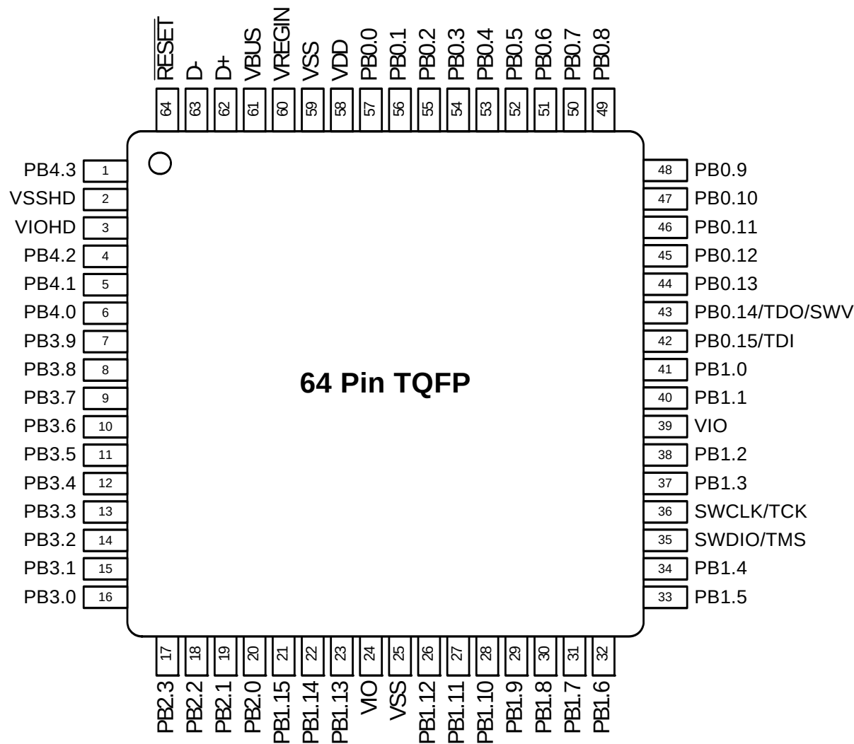
Figure 6.3. SiM3U1x6-GQ Pinout
