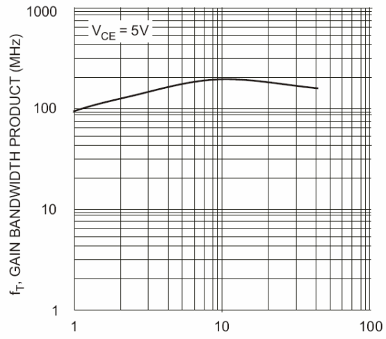
Fig. 4, Gain Bandwidth Product vs Collector Current
