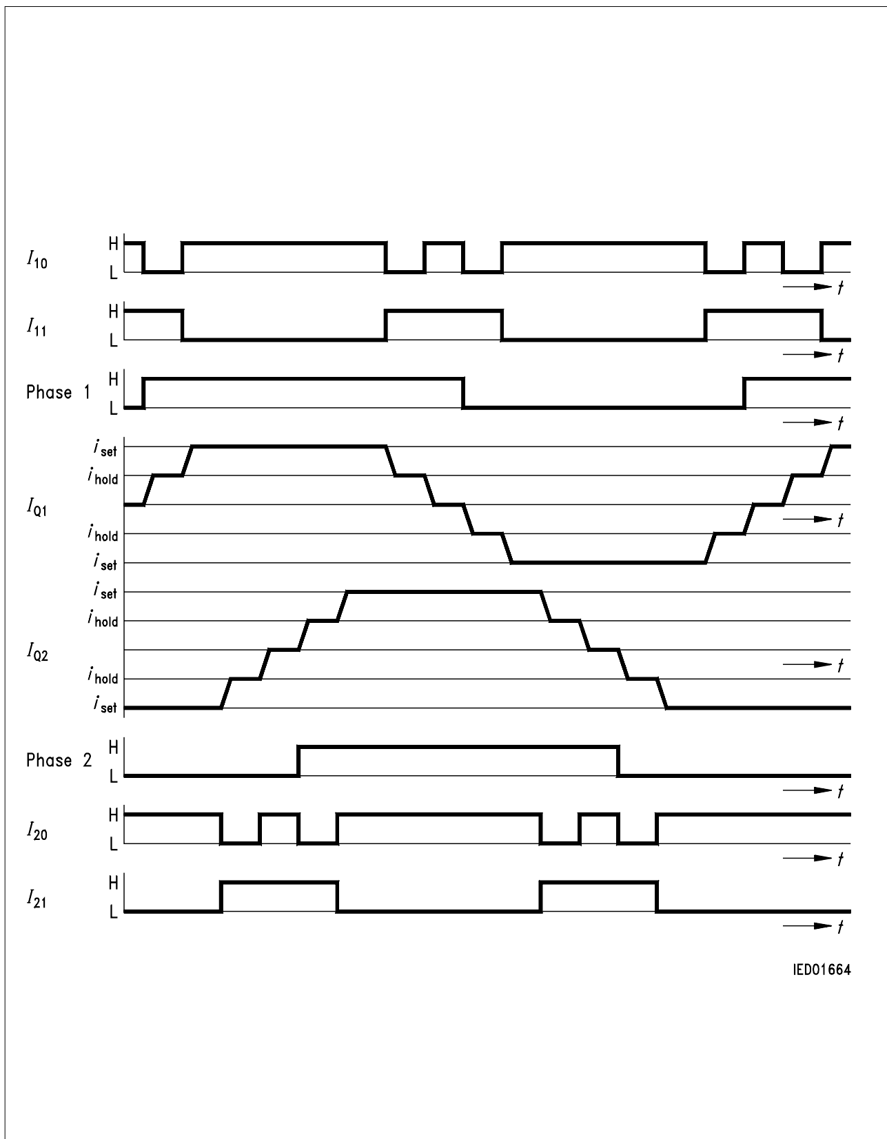
Figure 7 Quarter-Step Operation
