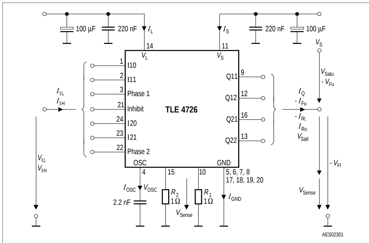
Figure 3 Test Circuit
