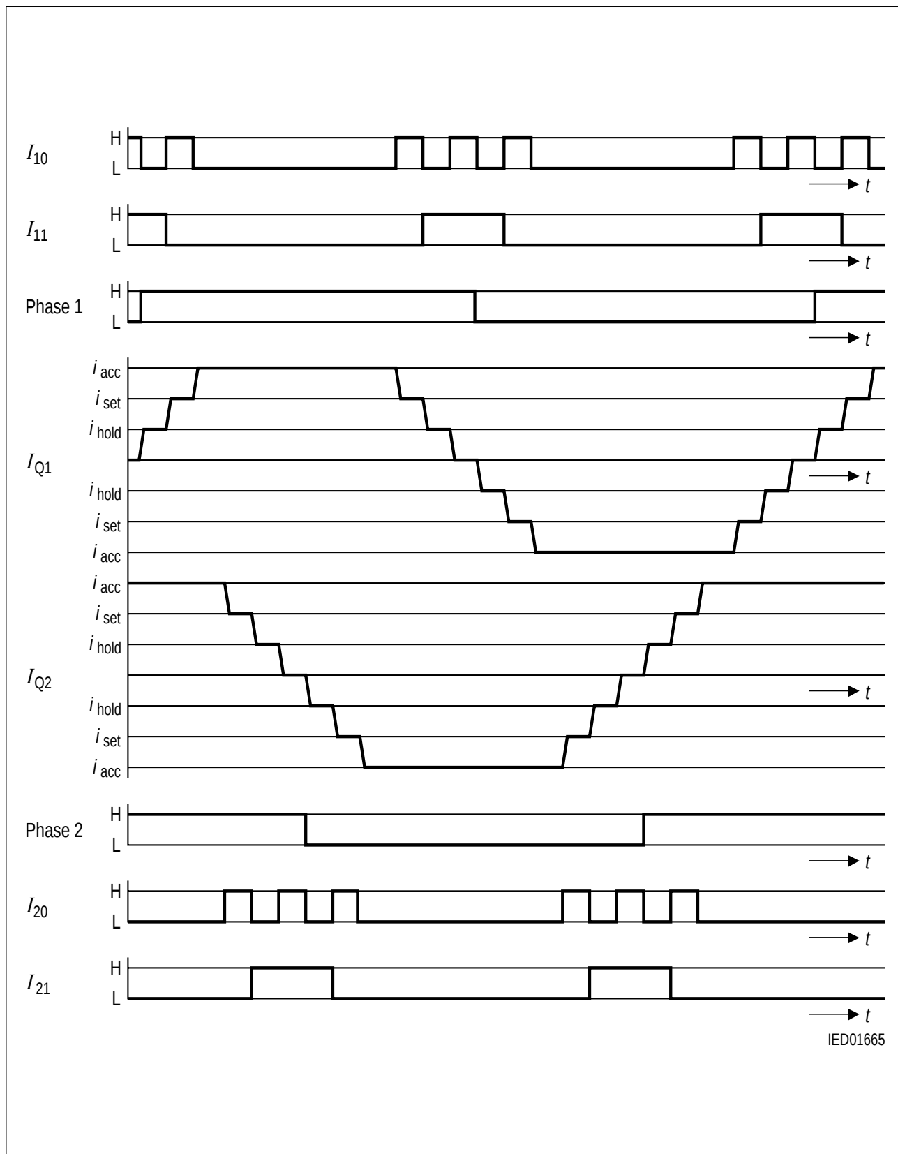
Figure 8 Mini-Step Operation
