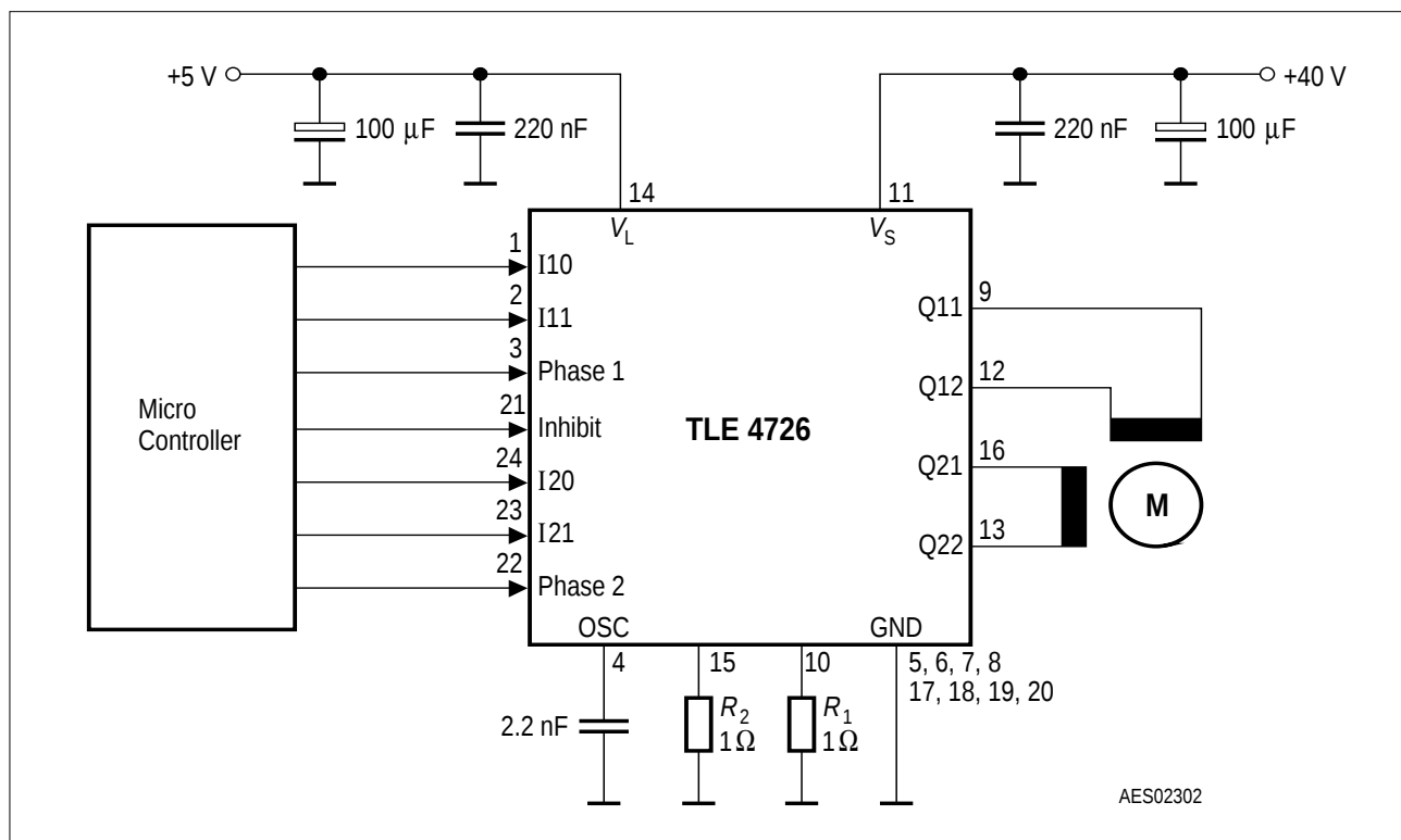
Figure 4 Application Circuit
