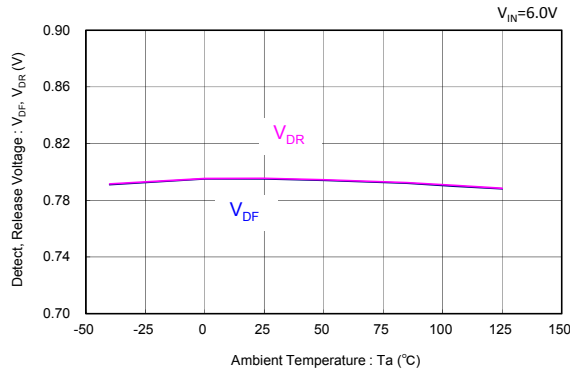
XC6134 ( V_{DF(T)}=0.8V )
