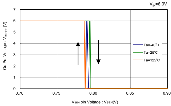
XC6134x08A ( V_{DF(T)}=0.8V )
