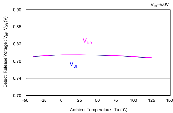
XC6134 ( V_{DF(T)}=0.8V )
