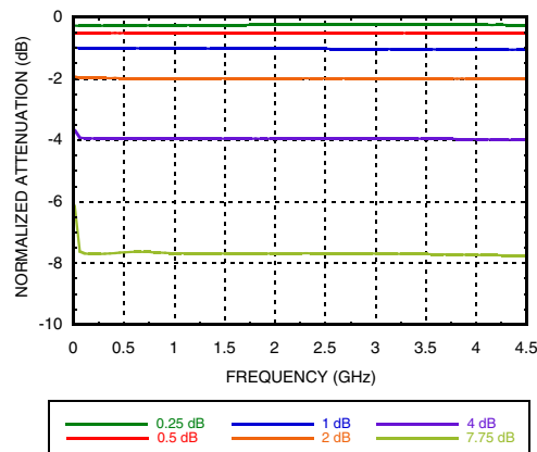
Normalized Attenuation (Only Major States are Shown)
