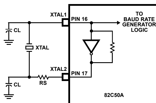
FIGURE 2. TYPICAL CRYSTAL OSCILLATOR CIRCUIT
