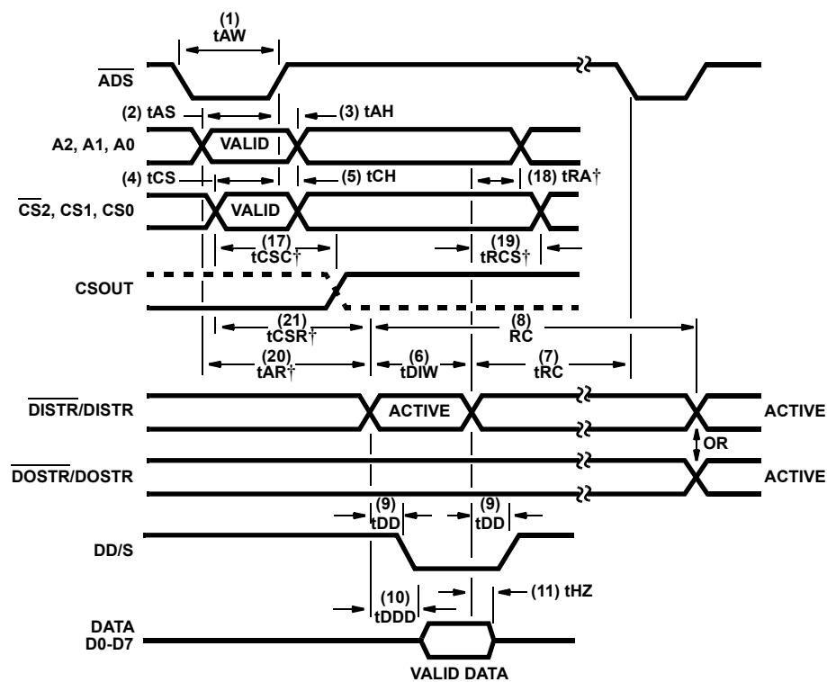
FIGURE 7. READ CYCLE
