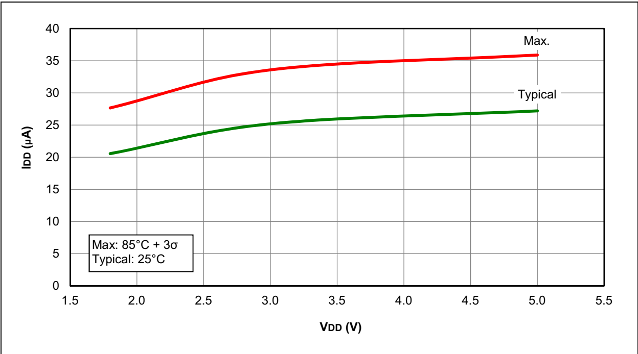
FIGURE 31-12: I_{DD} , LFINTOSC MODE ( F_{osc} = 31\text{ kHz} ), PIC16F1825/9 ONLY
