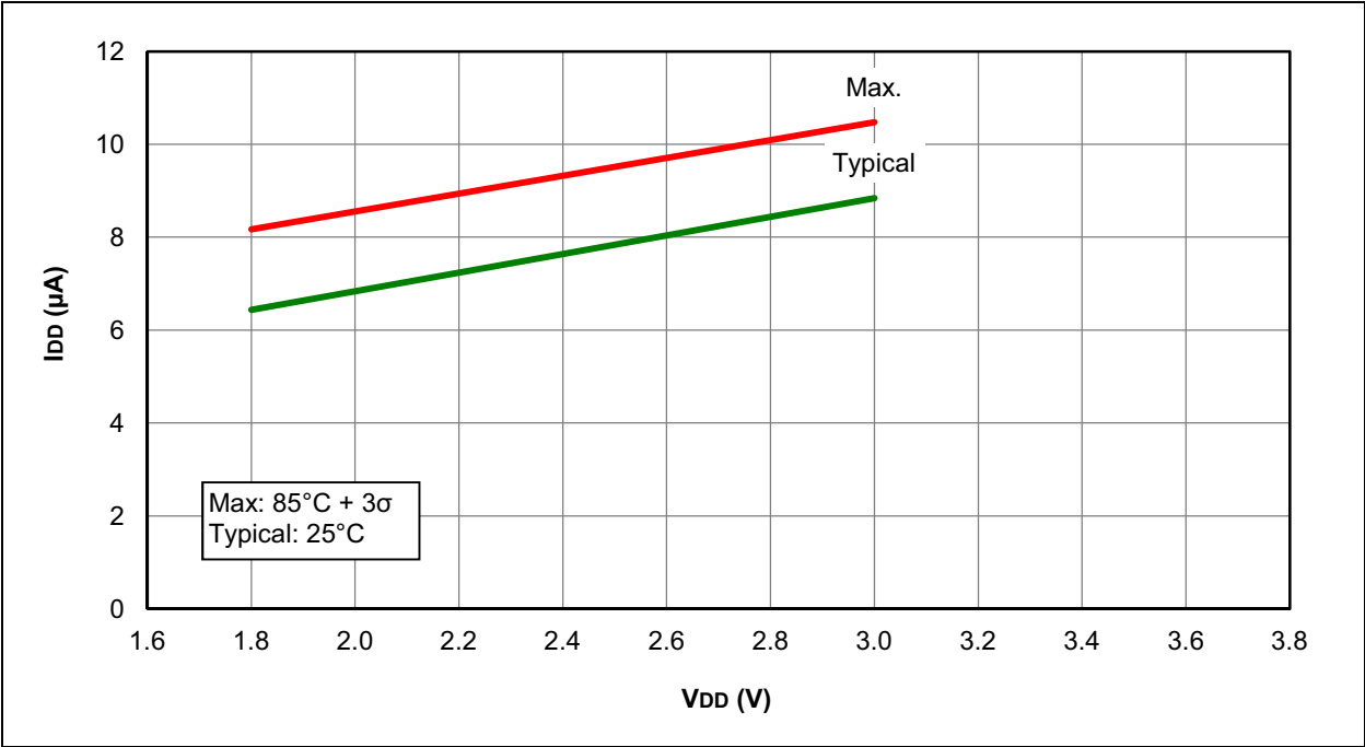
FIGURE 31-11: I_{DD} , LFINTOSC MODE ( F_{osc} = 31\text{ kHz} ), PIC16LF1825/9 ONLY
