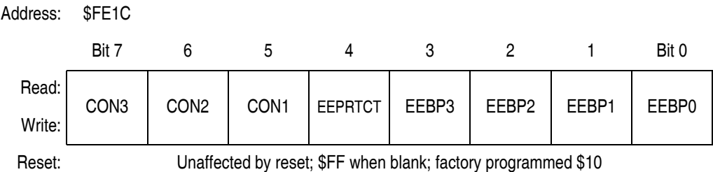
Figure 5-4. EEPROM Non-Volatile Register (EENVR)
