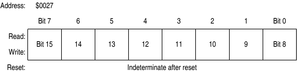
Figure 11-14. TIMA Channel 0 Register High (TACH0H)
