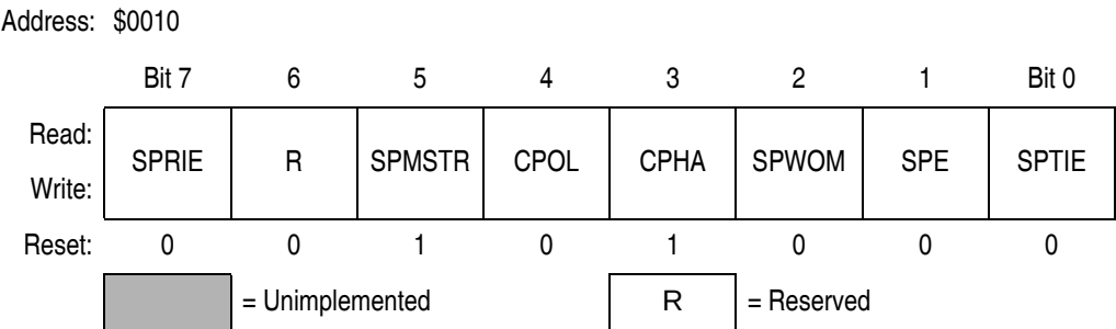
Figure 16-13. SPI Control Register (SPCR)
