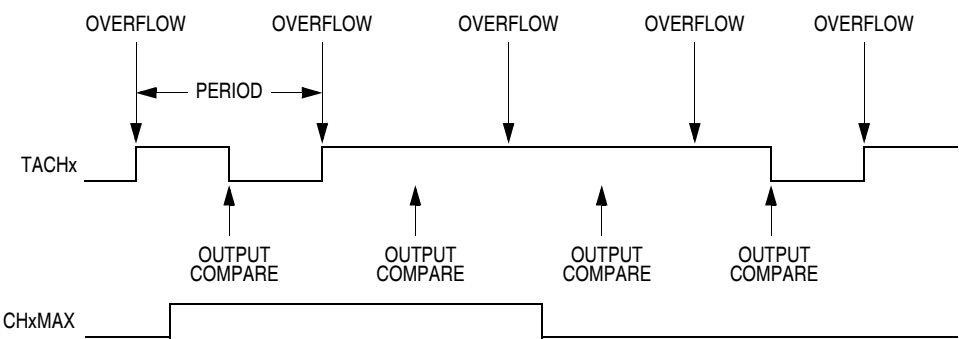
Figure 11-13. CHxMAX Latency
