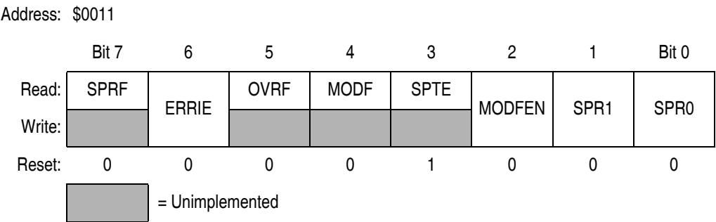
Figure 16-14. SPI Status and Control Register (SPSCR)
