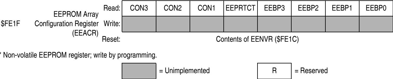
Figure 5-1. EEPROM I/O Register Summary
