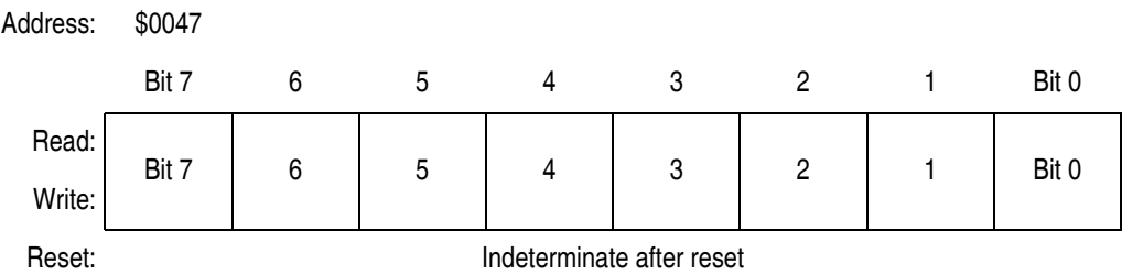
Figure 12-15. TIMB Channel 0 Register Low (TBCH0L)
