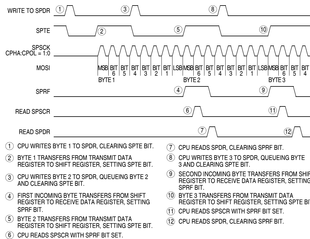
Figure 16-8. SPRF/SPTE CPU Interrupt Timing
