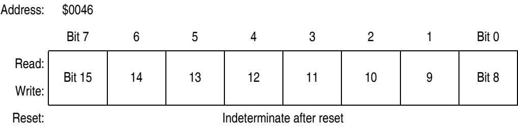
Figure 12-14. TIMB Channel 0 Register High (TBCH0H)
