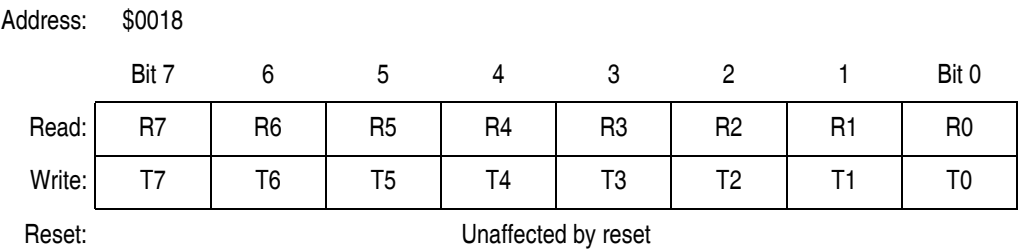
Figure 15-15. SCI Data Register (SCDR)
