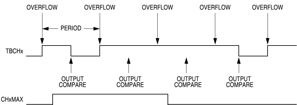
Figure 12-13. CHxMAX Latency
