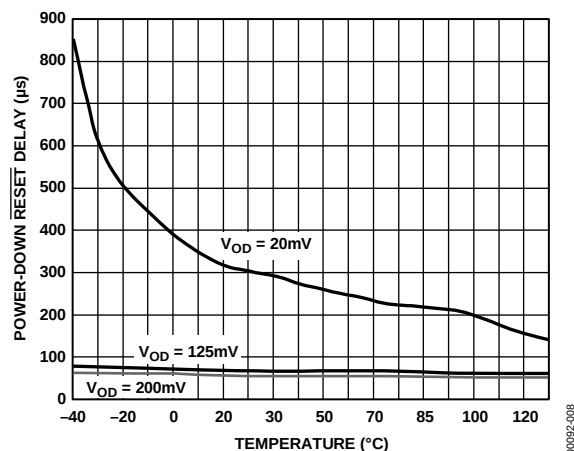
Figure 8. Power-Down \overline{RESET} Delay vs. Temperature (ADM81xL/M)
