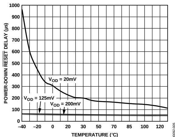
Figure 5. Power-Down \overline{RESET} Delay vs. Temperature (ADM81xR/S/T/Z)
