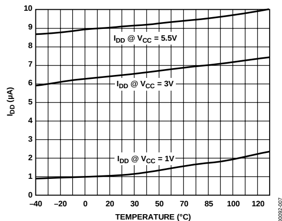
Figure 7. Supply Current vs. Temperature (ADM81xL/M)
