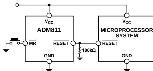
Figure 2. Typical ADM811 Operating Circuit
