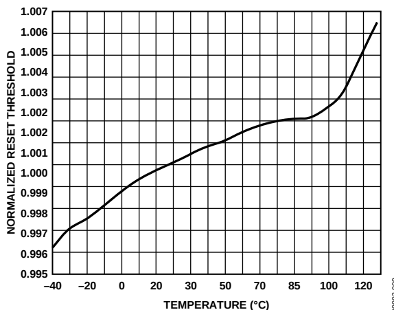
Figure 9. \overline{RESET} Threshold Deviation vs. Temperature
