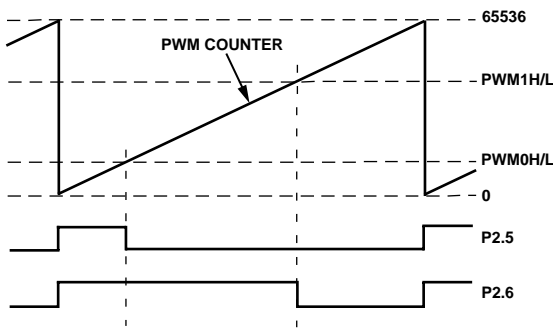
Figure 41. PWM Mode 3
