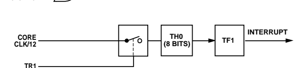
Figure 55. Timer/Counter 0, Mode 3
