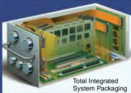
Space Application Connectors with Fiber Optics
