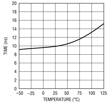
RS485 Receiver |t PLH - t PHL | vs Temperature
