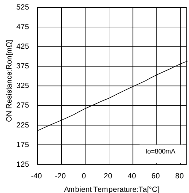
Figure 23. DCDC2 FET ON Resistance vs Temperature
