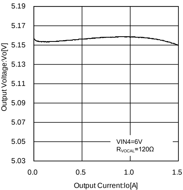
Figure 45. Voltage Adjusted for Cable Impedance vs Output Current
