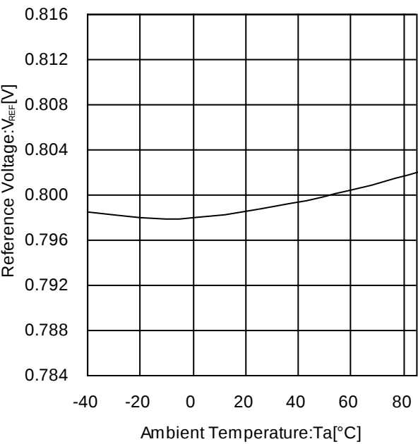
Figure 41. REG4 Reference Voltage vs Temperature
