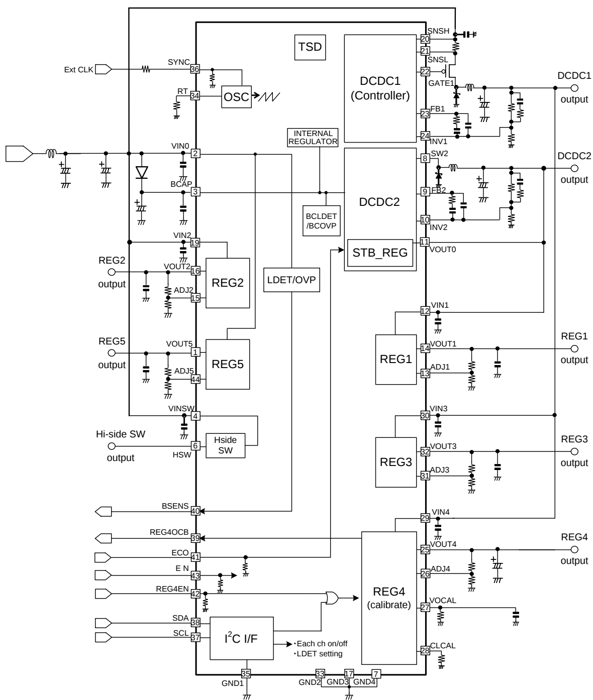
Figure 2. Block Diagram
