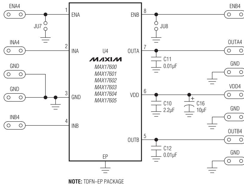
Figure 1d. MAX17600–MAX17605 EV Kit Schematic (U4)
