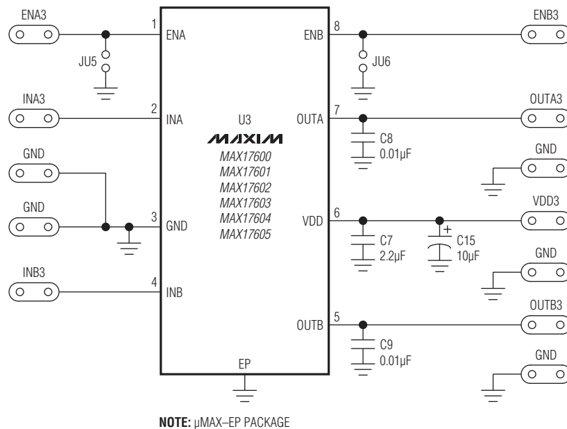
Figure 1c. MAX17600–MAX17605 EV Kit Schematic (U3)
