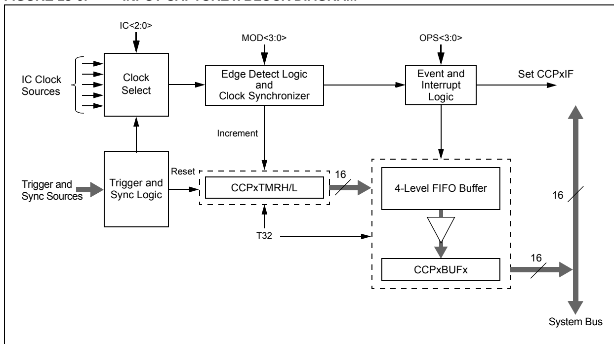
FIGURE 13-6: INPUT CAPTURE x BLOCK DIAGRAM
