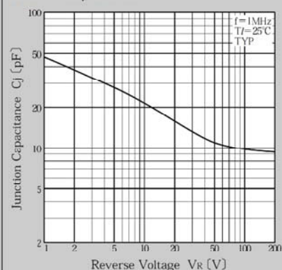
Junction Capacitance
